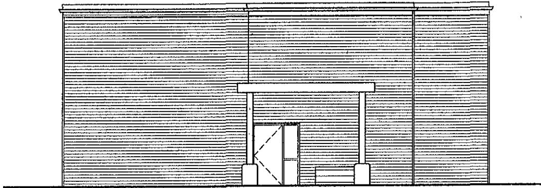
SIDE ELEVATION
