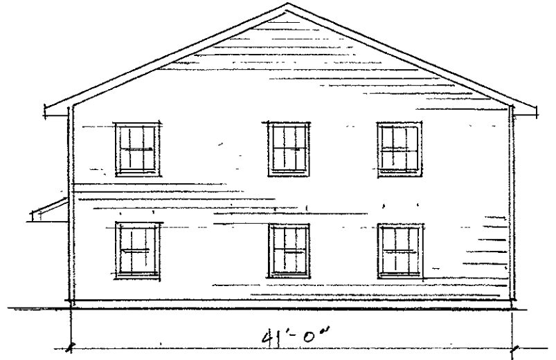
ERICKSON APARTMENTS SIDE ELEVATION - RIGHT
