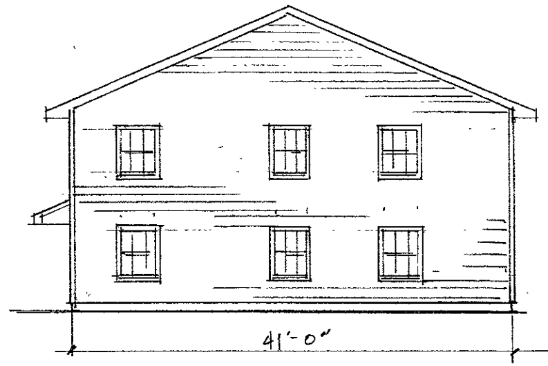
ERICKSON APARTMENTS SIDE ELEVATION - RIGHT
