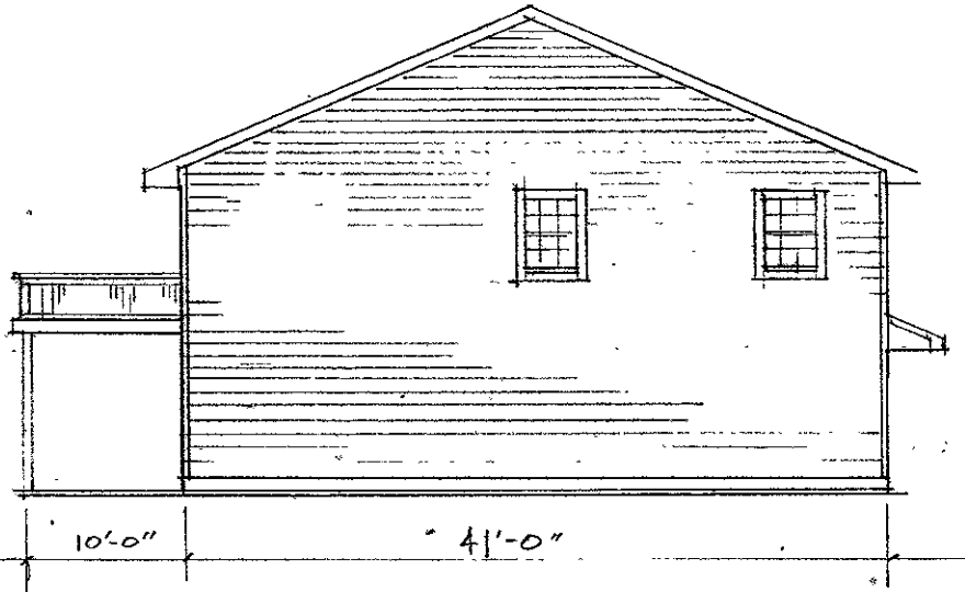
ERICKSON APARTMENTS SIDE ELEVATION - LEFT
