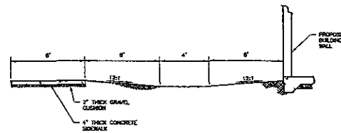
SIDEWALK / DITCH SECTION NOT TO SCALE
