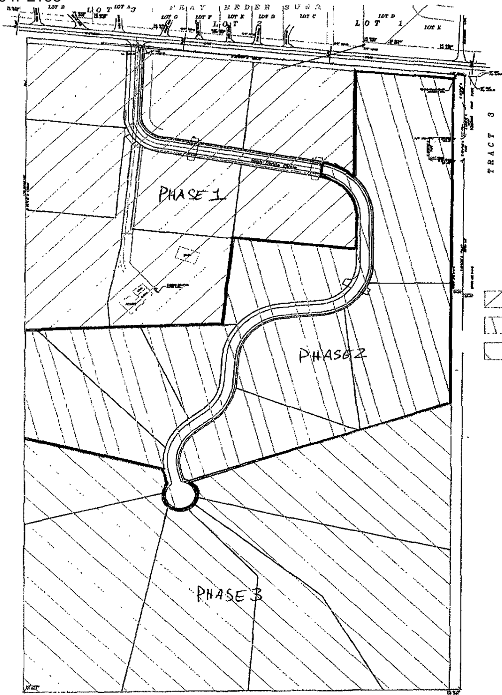
Phasing Plan
