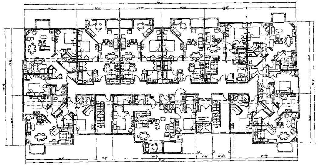
2 THIRD FLOOR PLAN 10-21-04
