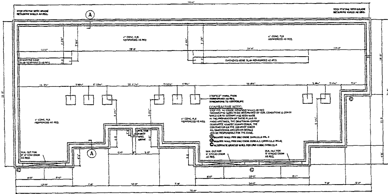
FTG./FND. PLAN SCALE: 1/4" = 1'-0" FOUNDATION 2068 SQ. FT.
