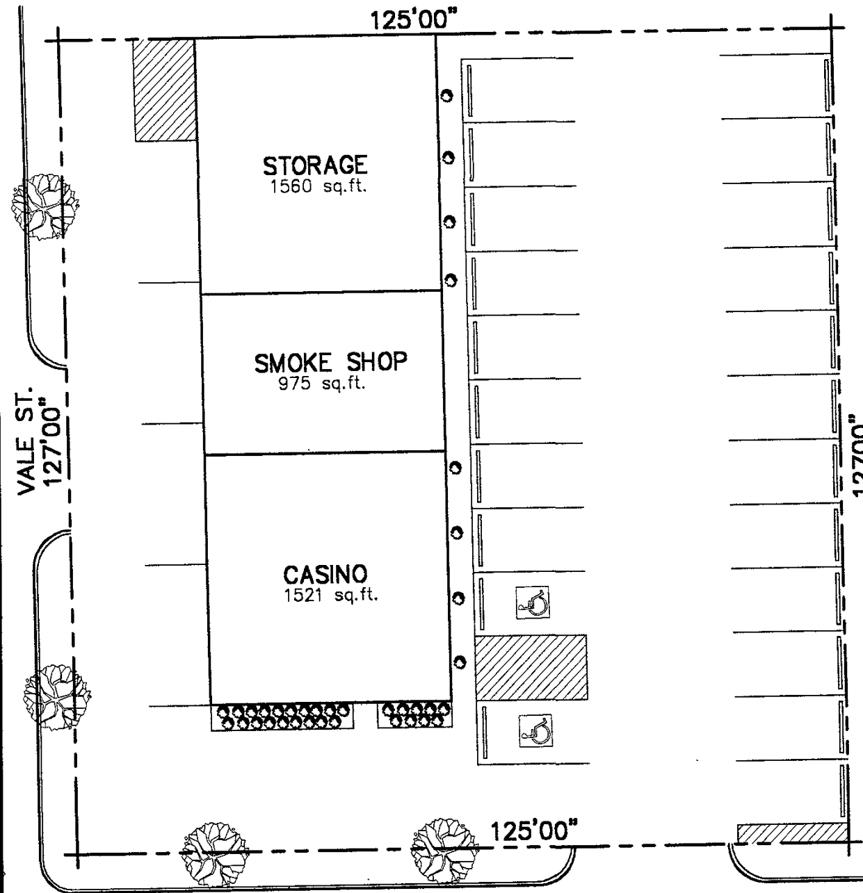
WEST MAIN ST. LANDSCAPE PLAN SCALE: 1"=20'
