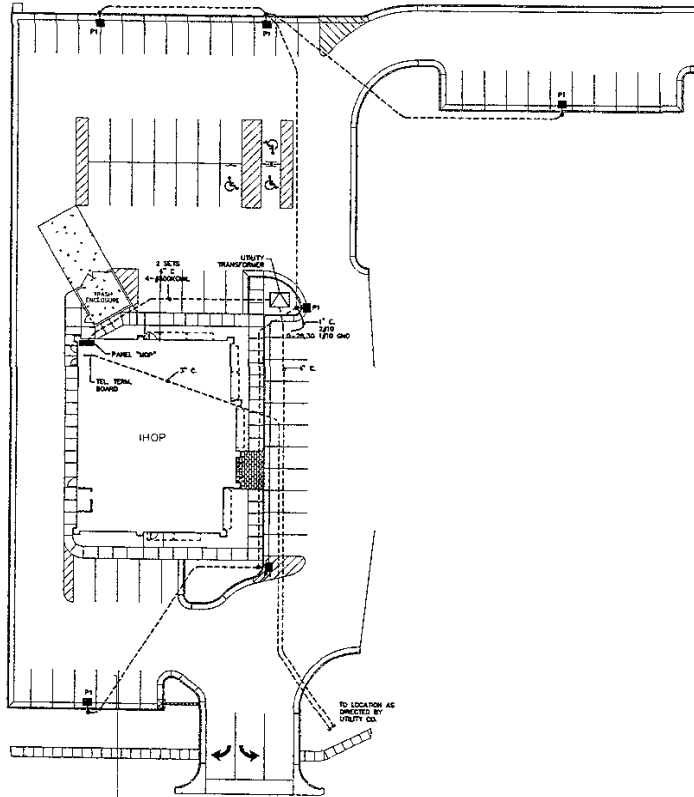
SITE PLAN - ELECTRICAL SCALE: 1"=20'-0"
