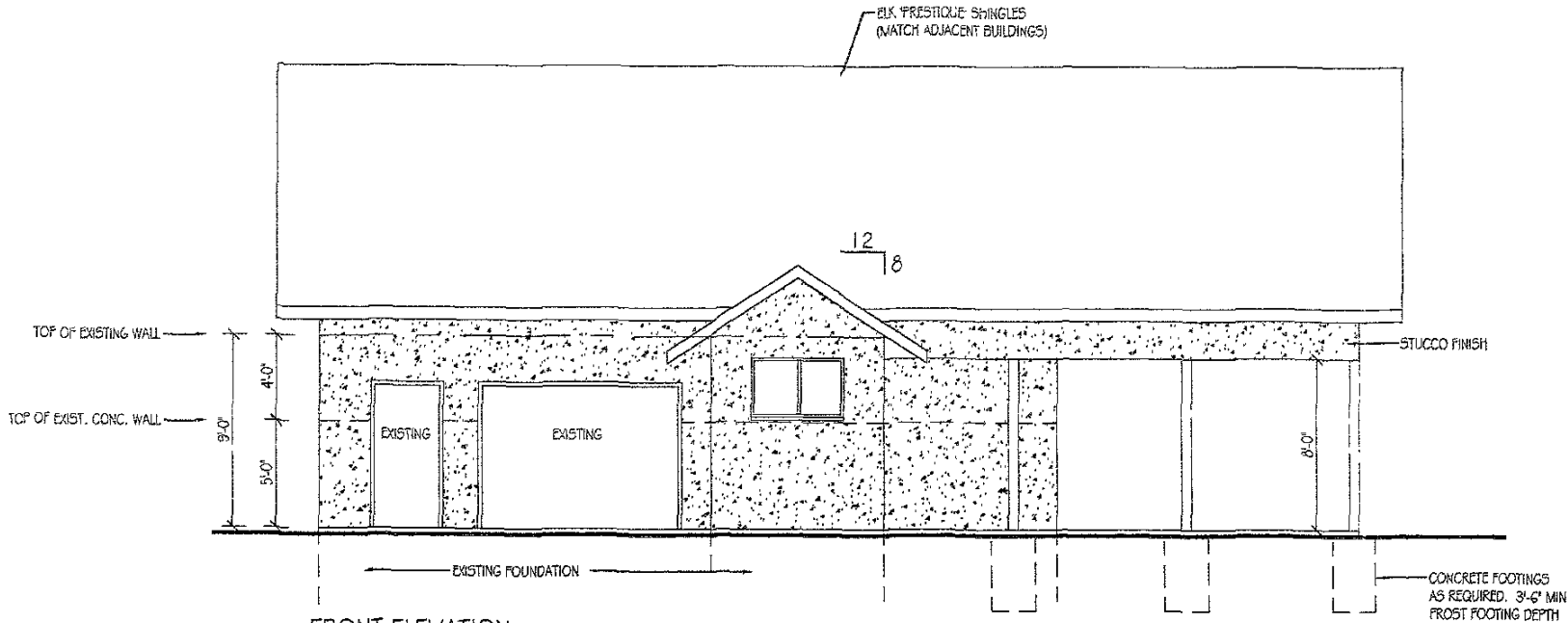
FRONT ELEVATION
