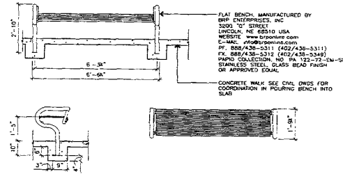
3 1.2 FLAT BENCH SCALE: 1/2" = 1'-0"
