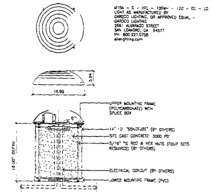
4 L4 DETAIL - MANTARAY WIDE FLOOD (M15) SCALE: 1 1/2" = 1'-0"
