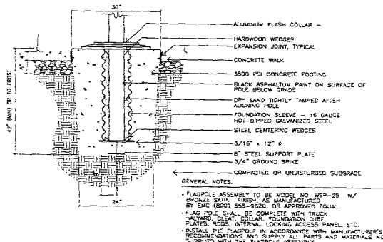
5 1.2 SECTION: FLAGPOLE FOOTING IN A CONCRETE WALK SCALE: 3/4" = 1'-0"
