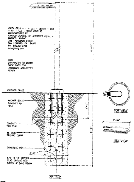
1 L4 DETAIL - AREA LUMINAIRES SCALE: 3/4" = 1'-0"
