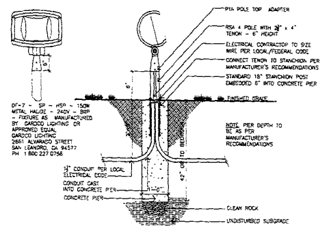
5 L4 SINGLE STANCHION MOUNT HORIZONTAL SPOT LIGHT SCALE: 3/4" = 1'-0"
