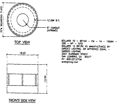
3 L4 DETAIL - BOLLARD (HEAD ONLY) SCALE: 1 1/2" = 1'-0"
