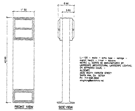
2 L4 DETAIL - SITE LIGHTING SCALE: 1 1/2" = 1'-0"
