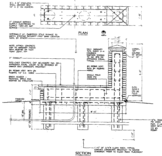
1 1.2 DETAIL: MONUMENT SIGN 'A' SCALE: 3/4" = 1'-0"
