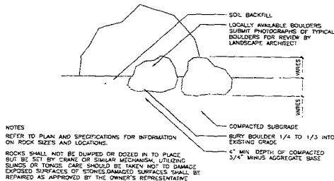
2 1.2 LANDSCAPE BOULDER PLACEMENT SCALE: 1" = 1'-0"
