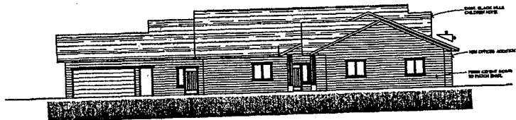
④ NORTHEAST ELEVATION 10'-7 1/2"
