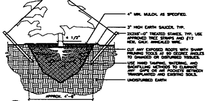
SECTION: TRANSPLANTED CONIFEROUS TREE NOT TO SCALE
