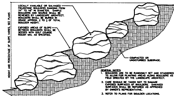
SECTION: TYPICAL BOULDER PLACEMENT ON SLOPE NOT TO SCALE
