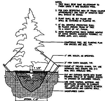
2 SECTION: TRANSPLANTED CONIFEROUS TREE NOT TO SCALE
