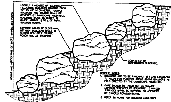
1 SECTION: TYPICAL BOULDER PLACEMENT ON SLOPE NOT TO SCALE
