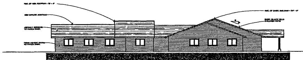
③ NORTHWEST ELEVATION 10' - 10"
