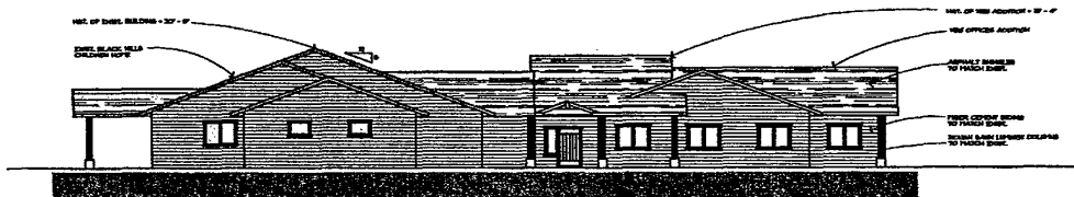
② SOUTHEAST ELEVATION 10' - 10"
