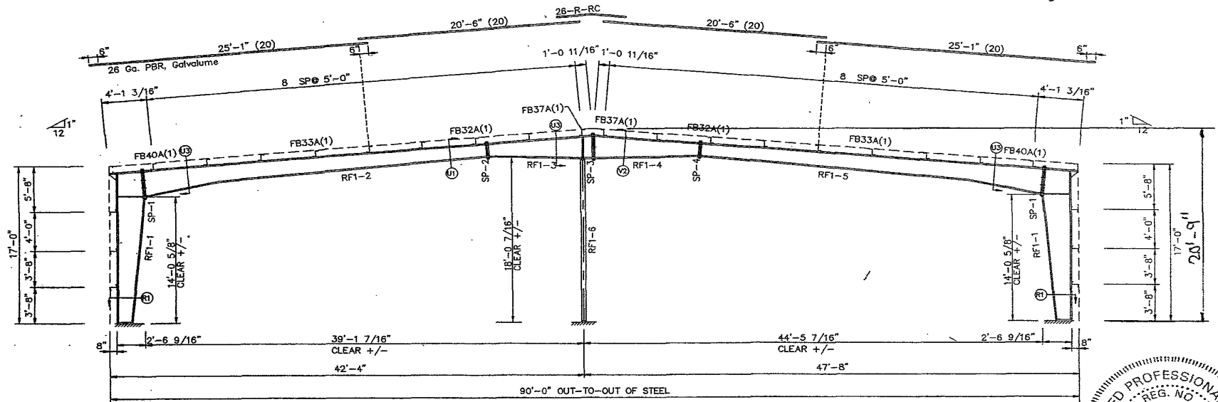
CROSS SECTION FOR FRAME LINE 1
