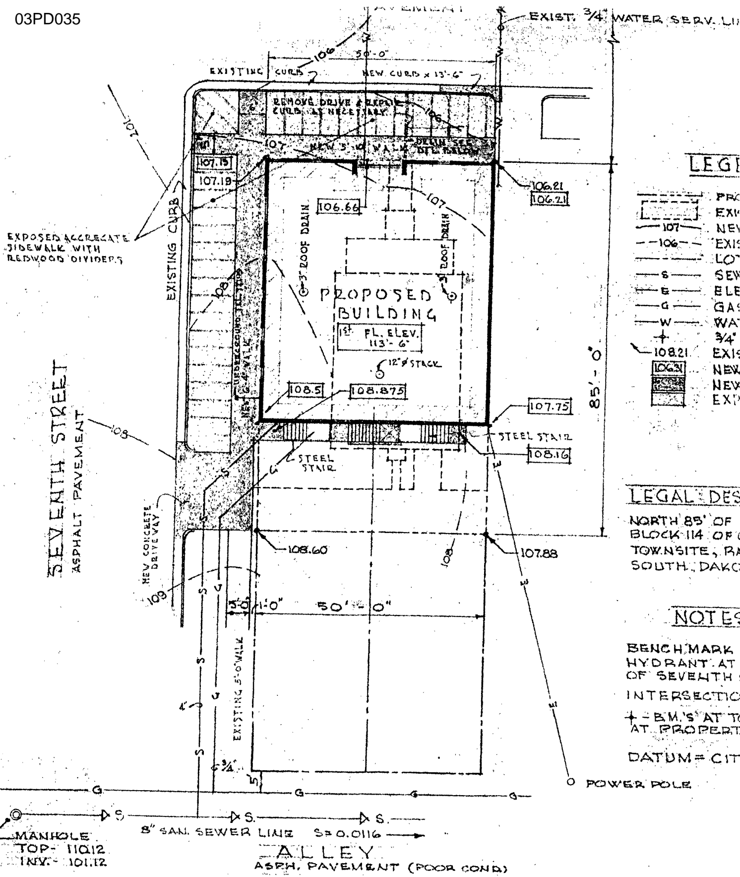
PLOT PLAN SCALE: 1" = 20'
