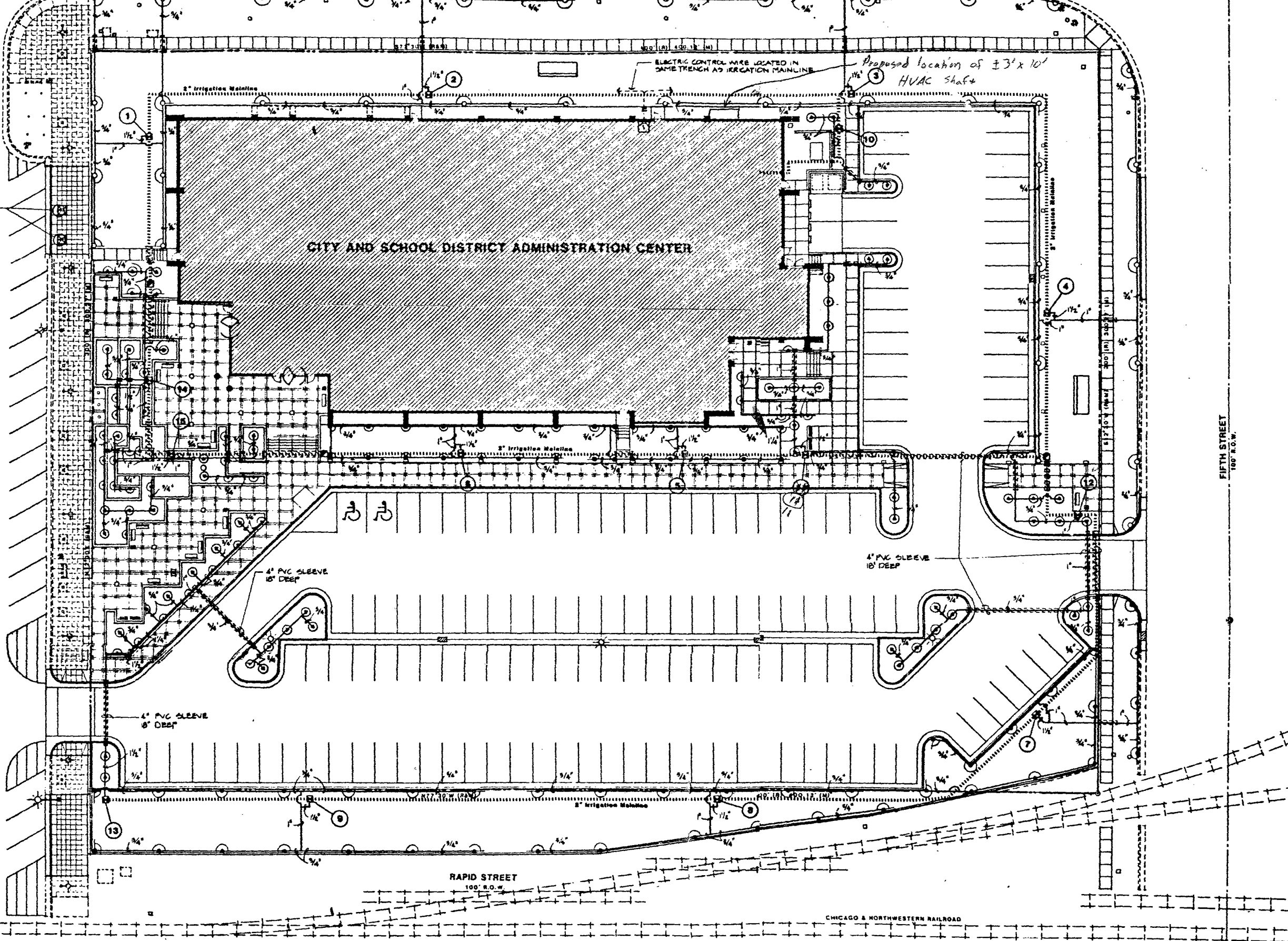
SITE IRRIGATION PLAN
