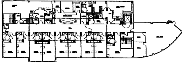
UPPER LEVEL FLOOR PLAN
