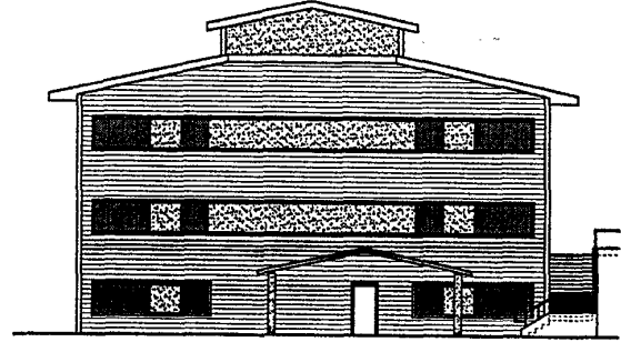
SOUTH ELEVATION SCALE 1/4" = 1'-0"
