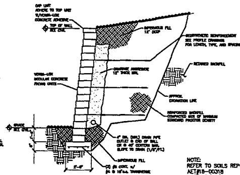
TYPICAL SECTION—REINFORCED RETAINING WALL SCALE: AS SHOWN
