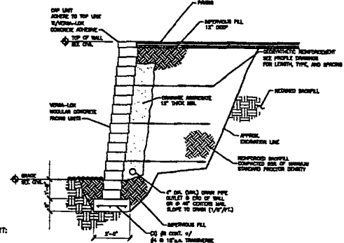
TYPICAL SECTION—REINFORCED RETAINING WALL SCALE: AS SHOWN
