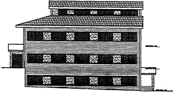
WEST ELEVATION SCALE 1/4" = 1'-0"
