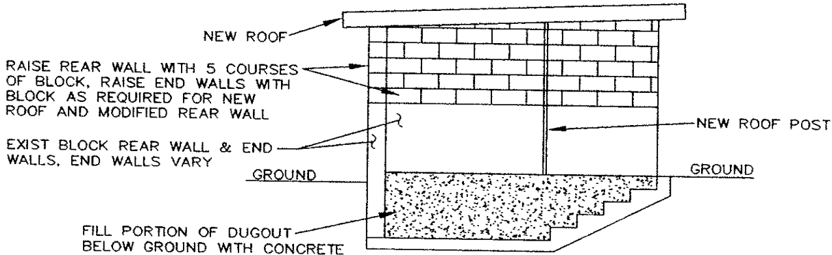
PROPOSED DUGOUT MODIFICATION -- CONCEPTUAL CROSS SECTION (NTS)
