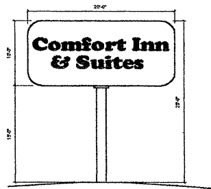
SIGNAGE - M-2
