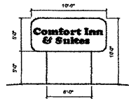
SIGNAGE - M-3
