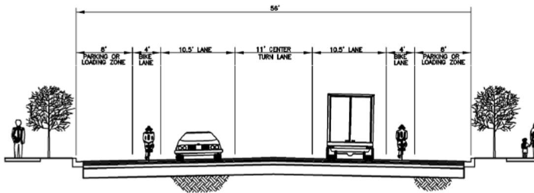
Figure 33. Proposed Highway 1416 Section with Bike Lanes.
