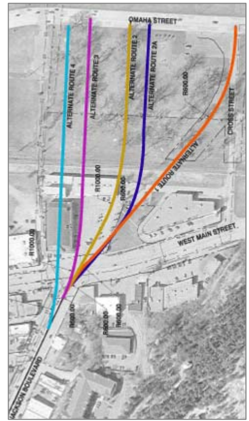
Figure 27. Jackson Boulevard Alignment Alternatives.
