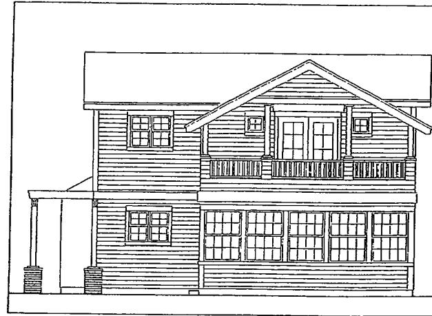
3 BACK ELEVATION 1/4"=1'-0"
