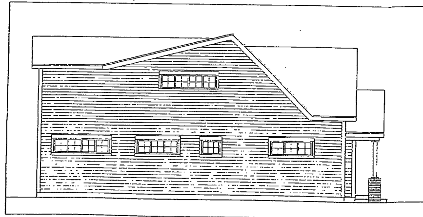
5 WEST ELEVATION A2.1 1/4"=1'-0"
