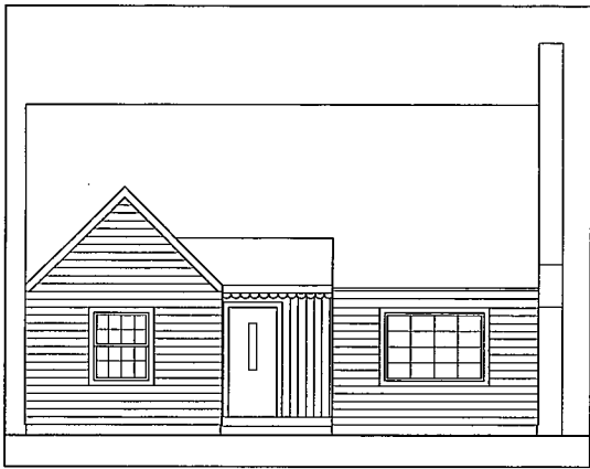
1 FRONT ELEVATION-BEFORE A2.1 1/4"=1'-0"
