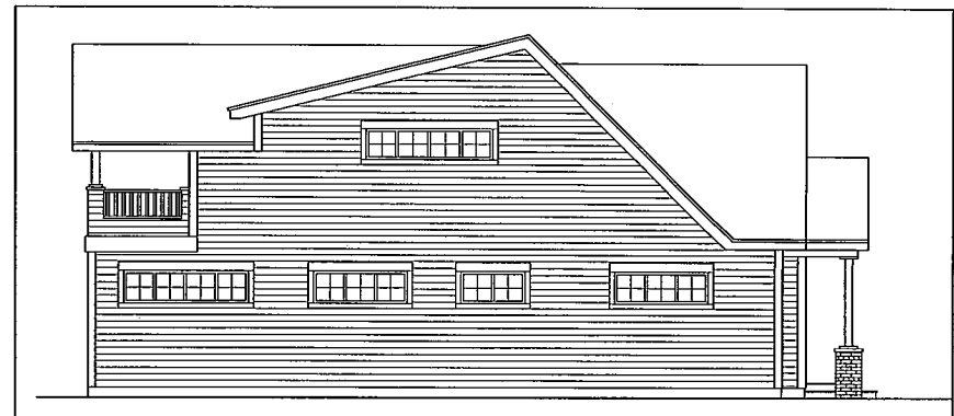
5 WEST ELEVATION A2.1 1/4"=1'-0"
