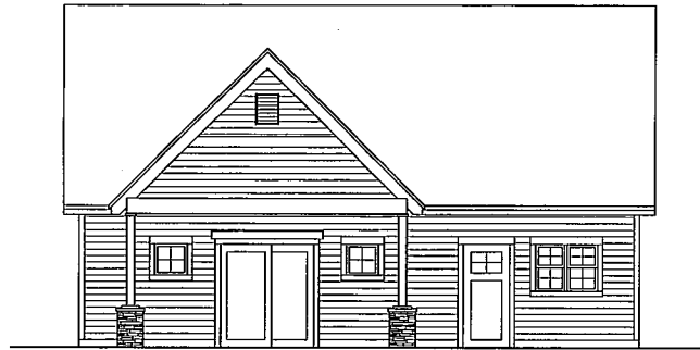
1 SOUTH ELEVATION A3.1 1/4"=1'-0"
