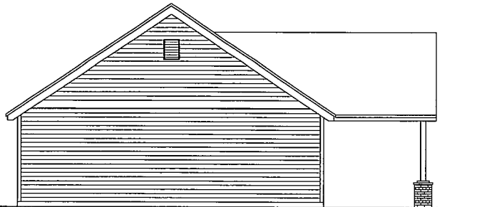
3 WEST ELEVATION A3.1 1/4"=1'-0"
