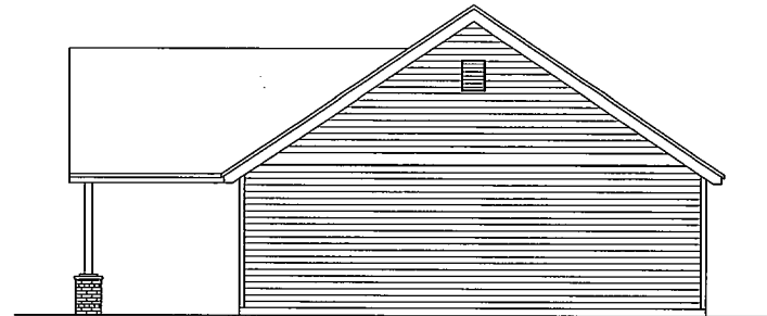
4 EAST ELEVATION A3.1 1/4"=1'-0"
