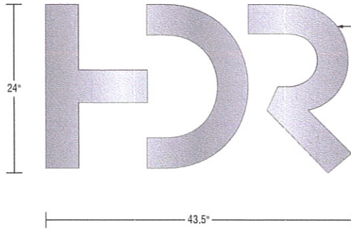
A Project Detail - Option 2 SCALE 3/4" = 1'-0"
