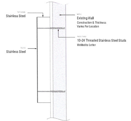
C Typical Mounting Section NTS
