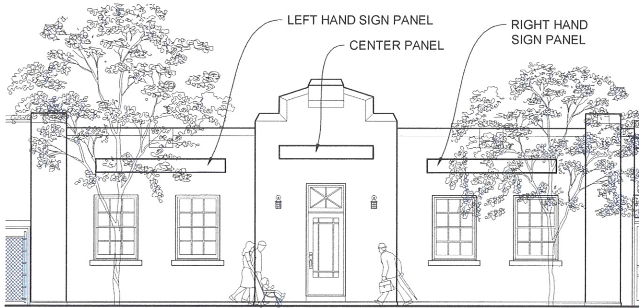
MAIN STREET ELEVATION \frac{1}{8}'' = 1'-0''
