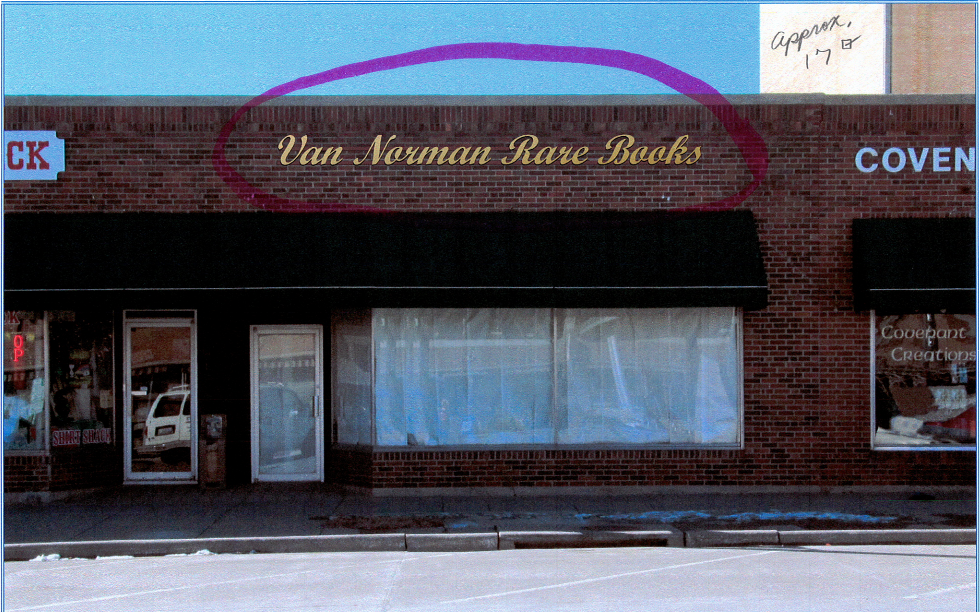
9" - 15" routed 1/2" mdx letters painted metallic gold, mounted on rails (17' 9") painted to match brick
