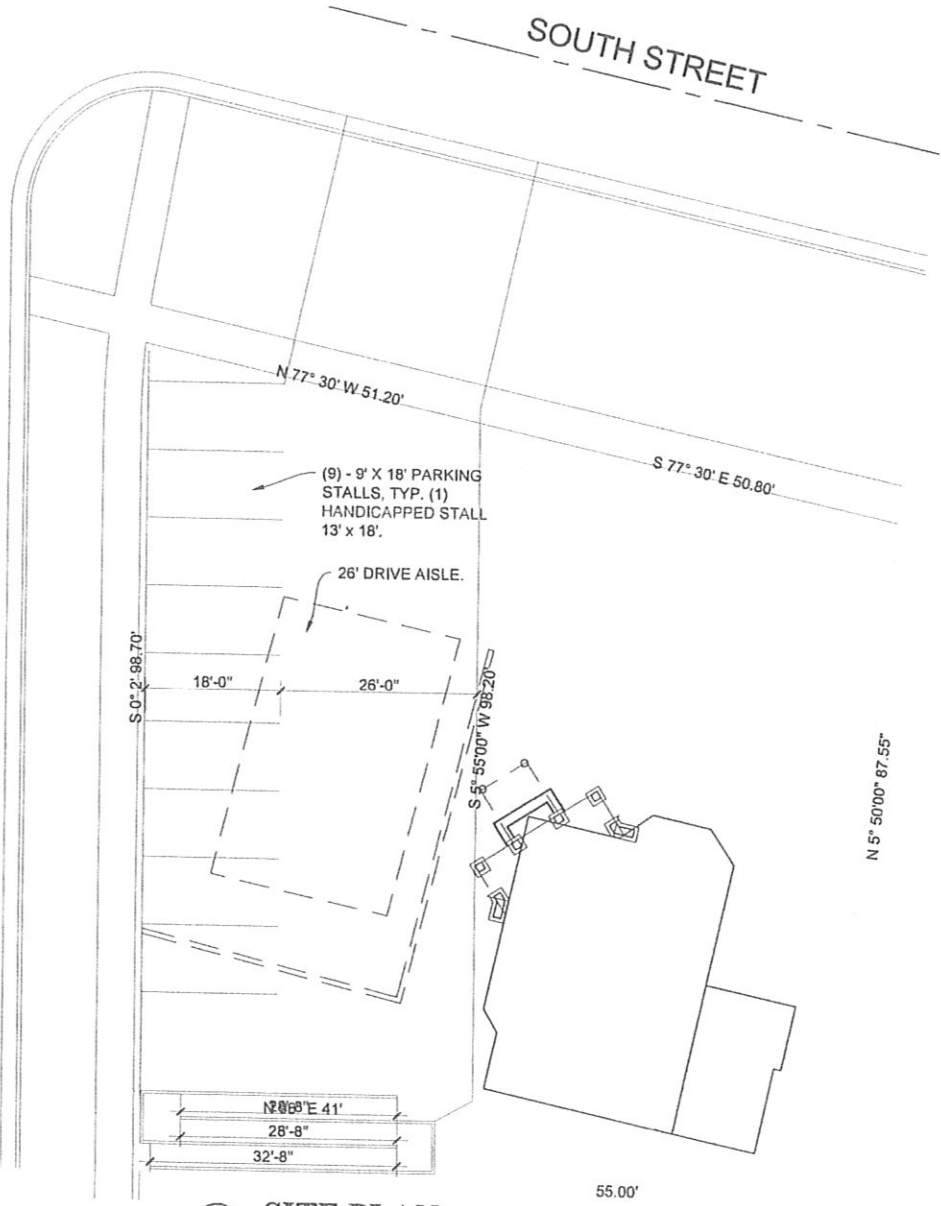
A SITE PLAN SCALE: 1/16" = 1'-0"
