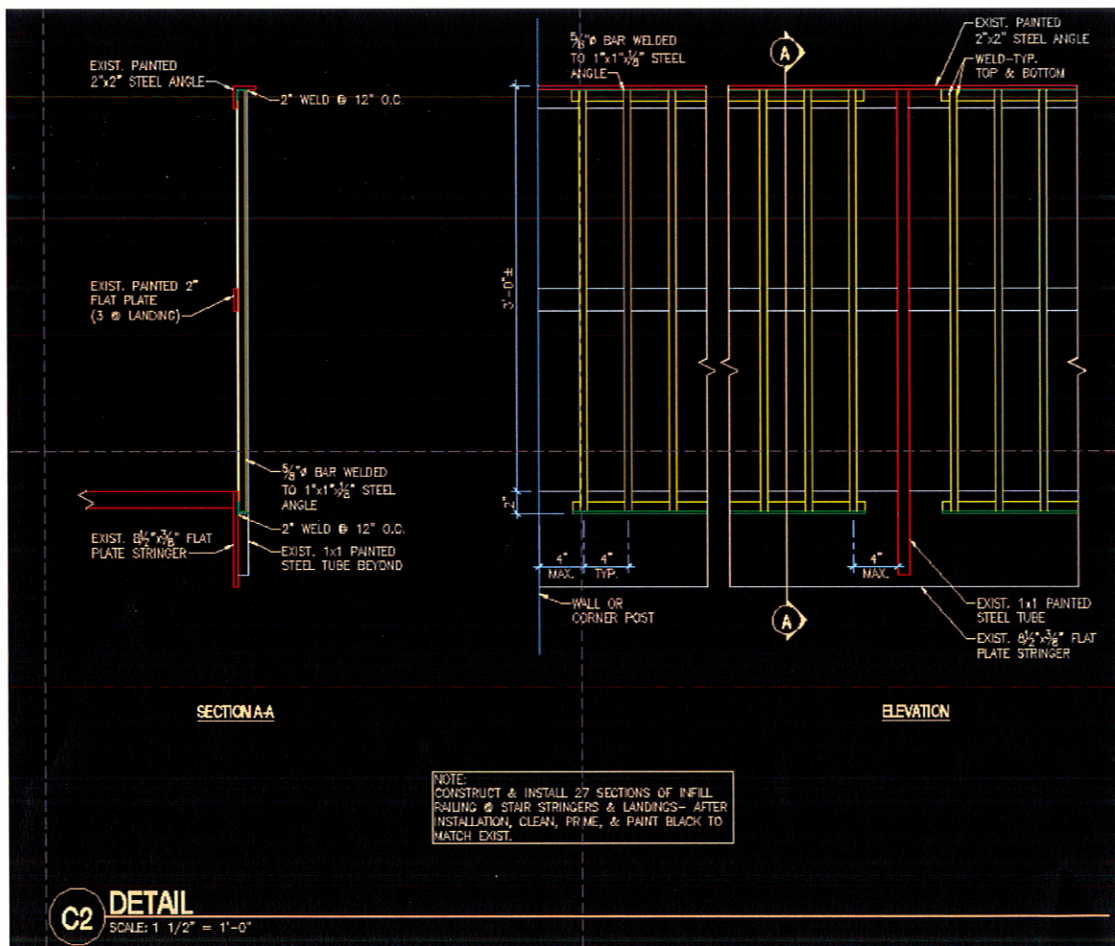
Detail C2 of the Construction Documents
