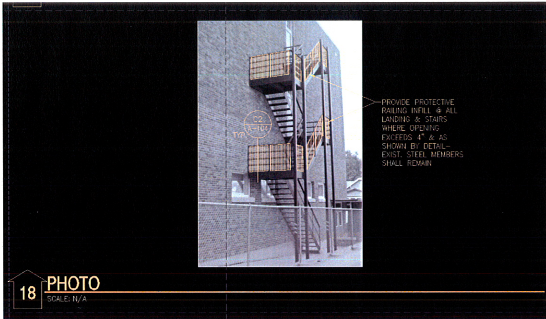
Detail 18 of the Construction Documents
