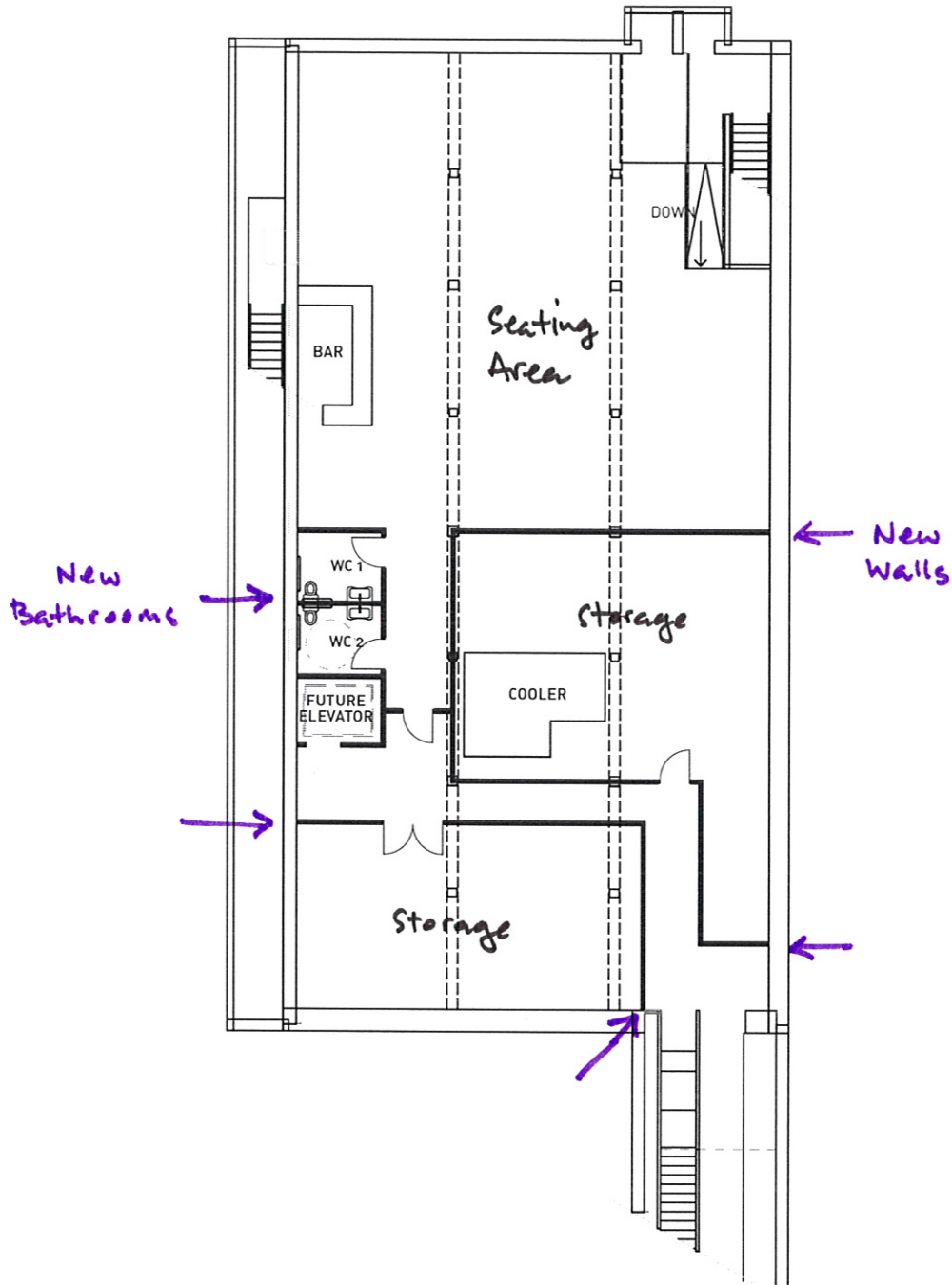
1 LOWER LEVEL FLOOR PLAN A1.1 SCALE: 1/8" = 1'-0"
