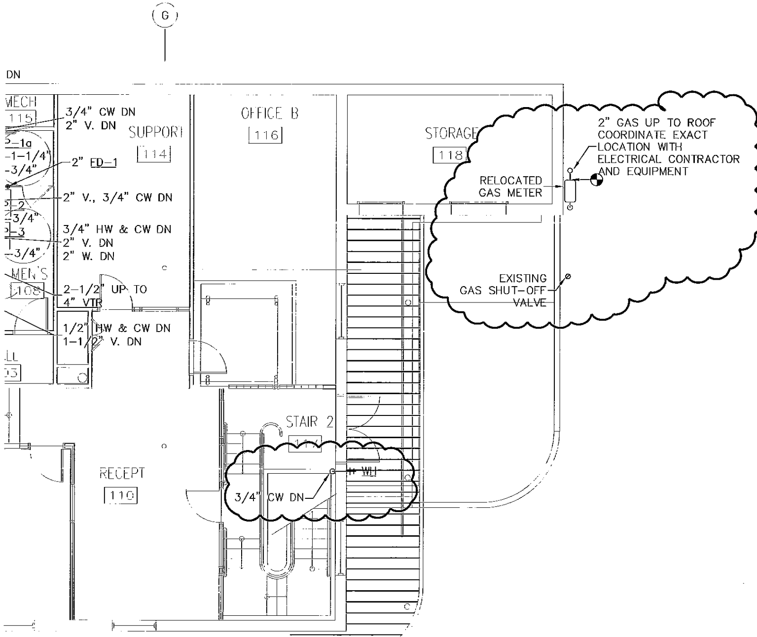
1 FIRST FLOOR PLUMBING PLAN SCALE 1/8" = 1'-0"
