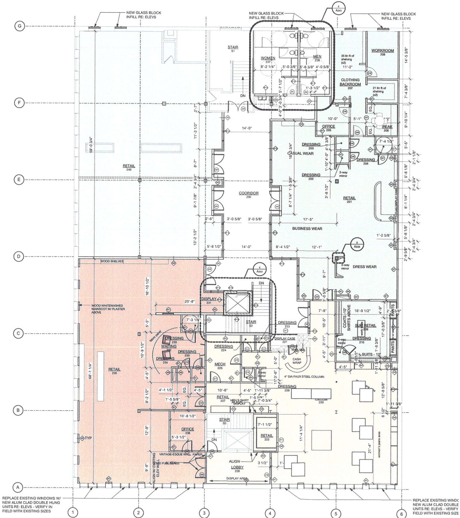
1 Second Floor Plan A2.0 Scale 1/8 = 1'-0"
