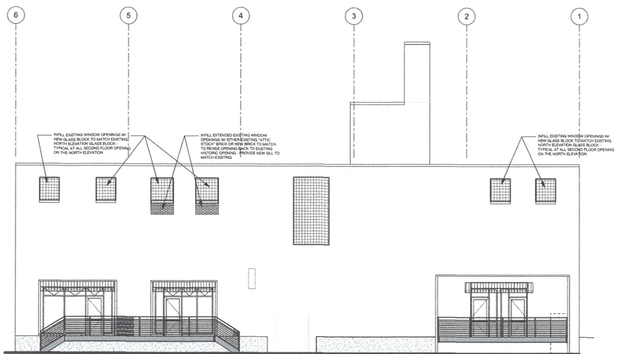
1 North Elevation A3.0 Scale 1/8" = 1'-0"
