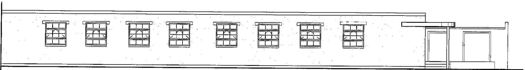
WEST ELEVATION
