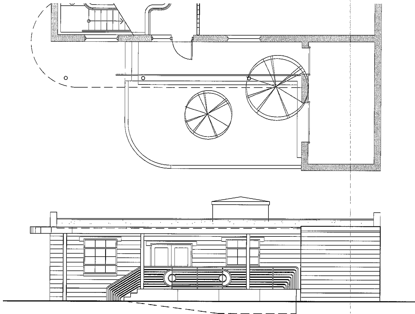
REAR ENTRY: plan + elevation
