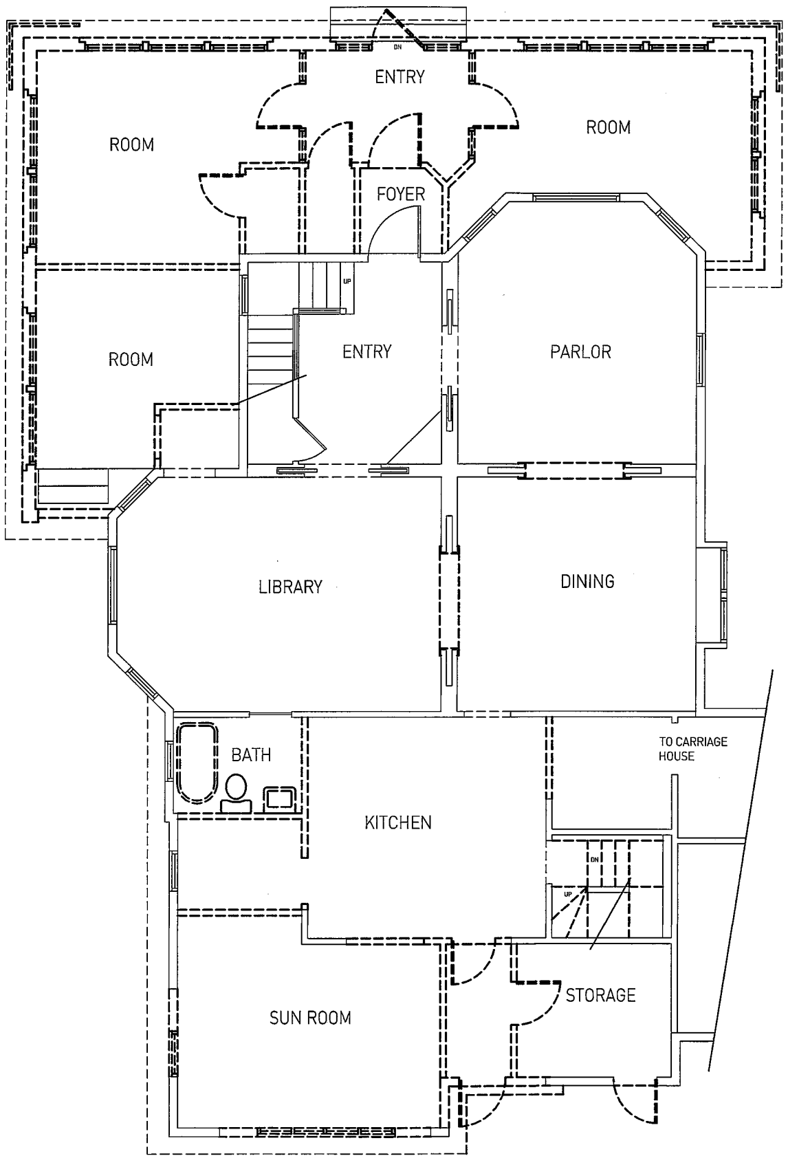
1 FIRST FLOOR PLAN - DEMOLITION
