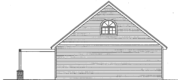
4 EAST ELEVATION A6.1 1/4"=1'-0"
