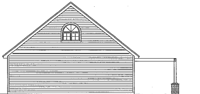
3 WEST ELEVATION A6.1 1/4"=1'-0"
