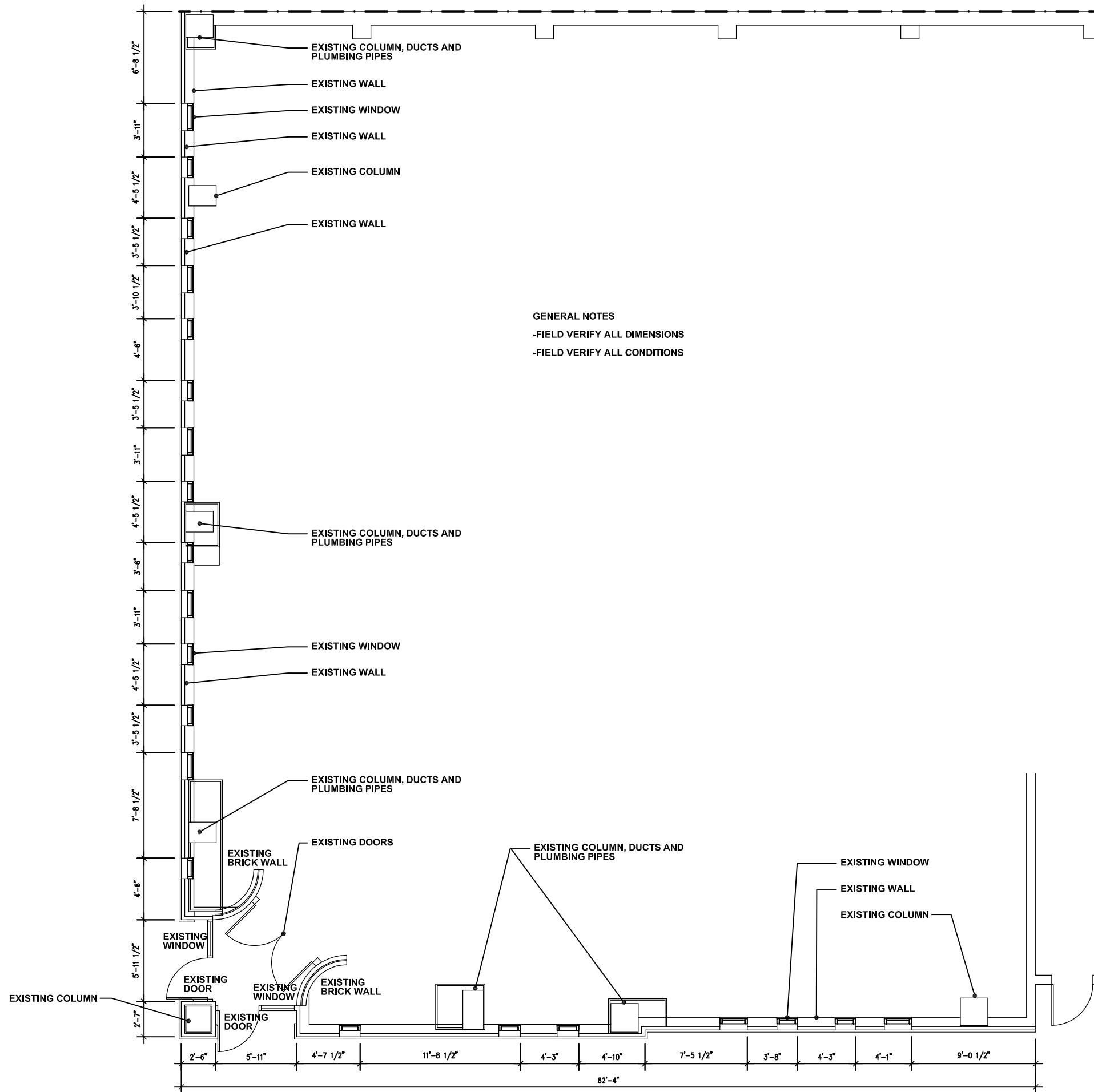
PARTIAL EXISTING FLOOR PLAN SCALE: 1/8" = 1'-0"
