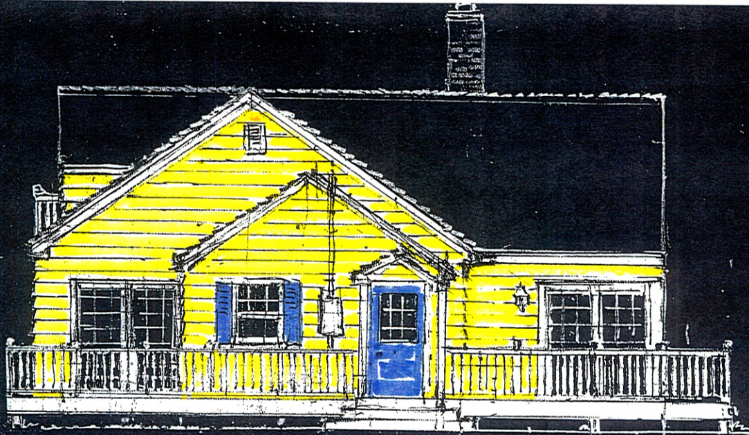
SOUTH ELEVATION SCALE \frac{1}{8}=1"
