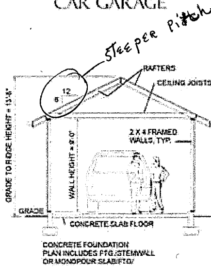
CROSS-SECTION
