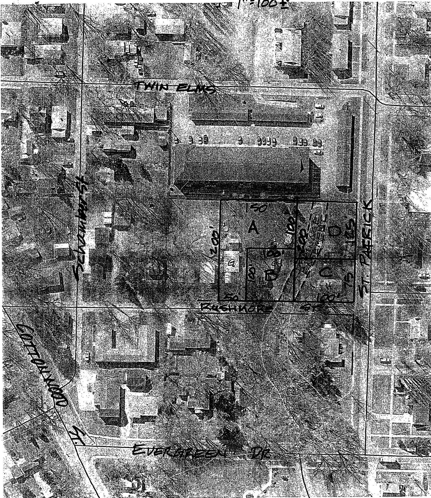
PLAT OF LOTS A, B, C, AND D (formerly Lots 16, 17, 18, 19 and 20) of Block 3 of Schamber Addition located in the NW 1/4 of NE 1/4, Section 9, T1N, R7E, BHM, Rapid City, Pennington County, South Dakota
