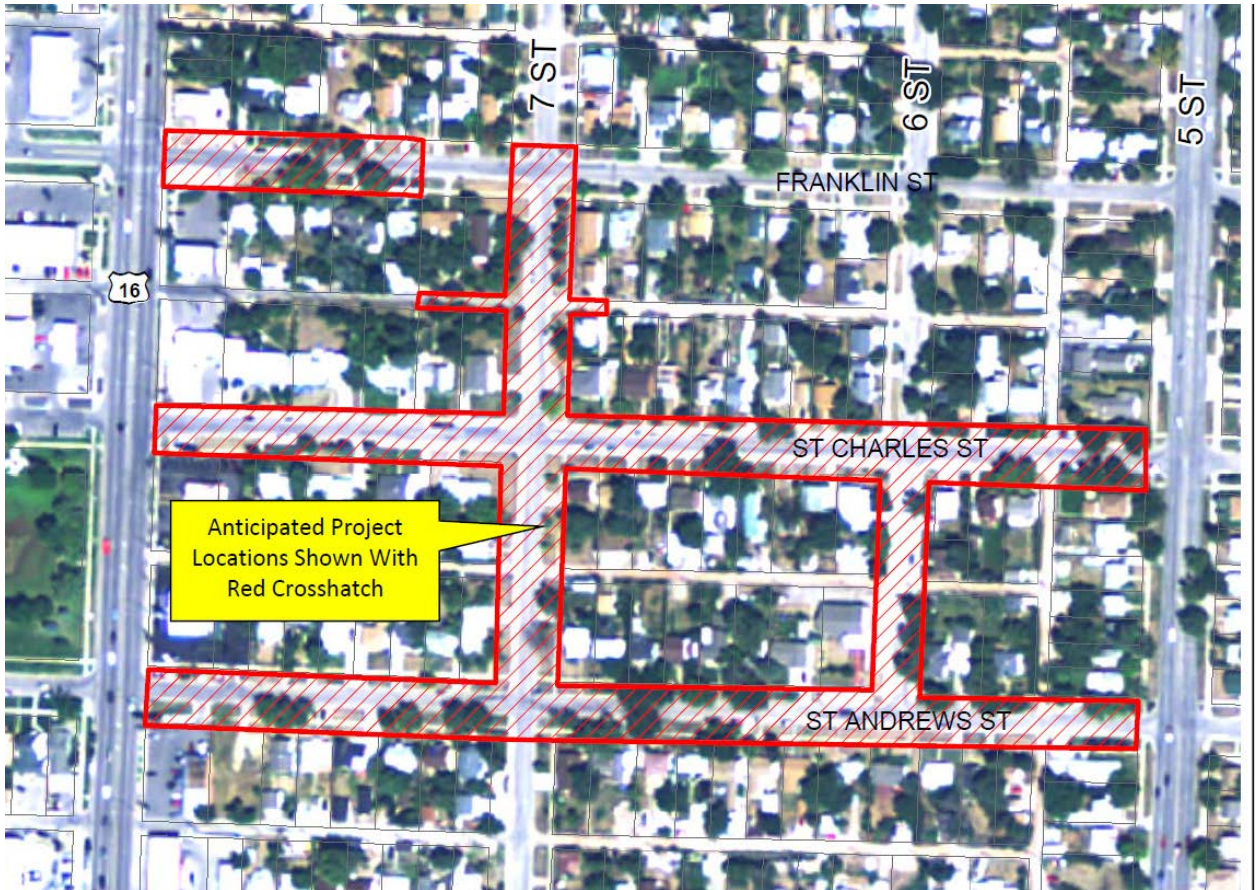
SAINT ANDREW STREET AND SAINT CHARLES STREET SANITARY SEWER AND WATER EXTENSION & RECONSTRUCTION
