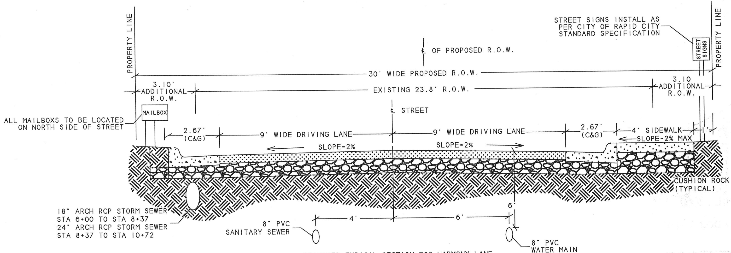
PROPOSED TYPICAL SECTION FOR HARMONY LANE STATION 0+00.00 TO STATION 10+58.04 N.T.S.
