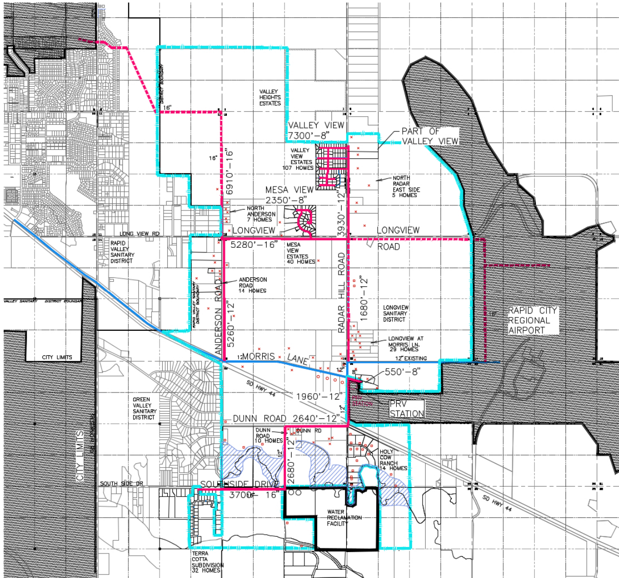
FIGURE 4 - PROPOSED WATER DISTRIBUTION SYSTEM FOR EAST RAPID CITY WATER EXPANSION
