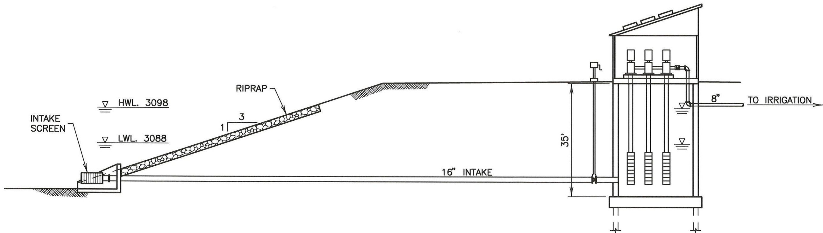
FIGURE 6 SCHEMATIC DESIGN BOX ELDER CREEK ALLUVIUM
