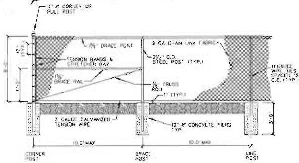
CHAIN LINK FENCE DETAIL NOTES
