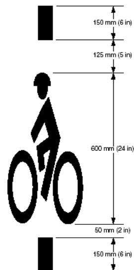
Recommended loop detector marking design.
