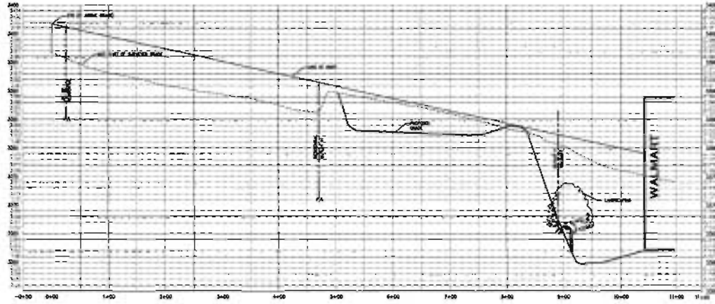
SIGHT LINE LOT 8B scale: 1"=60' horizontal 1"=6' vertical
