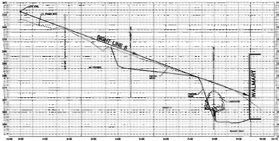
SIGHT LINE 5 scale: 1"=60' horizontal 1"=6' vertical
