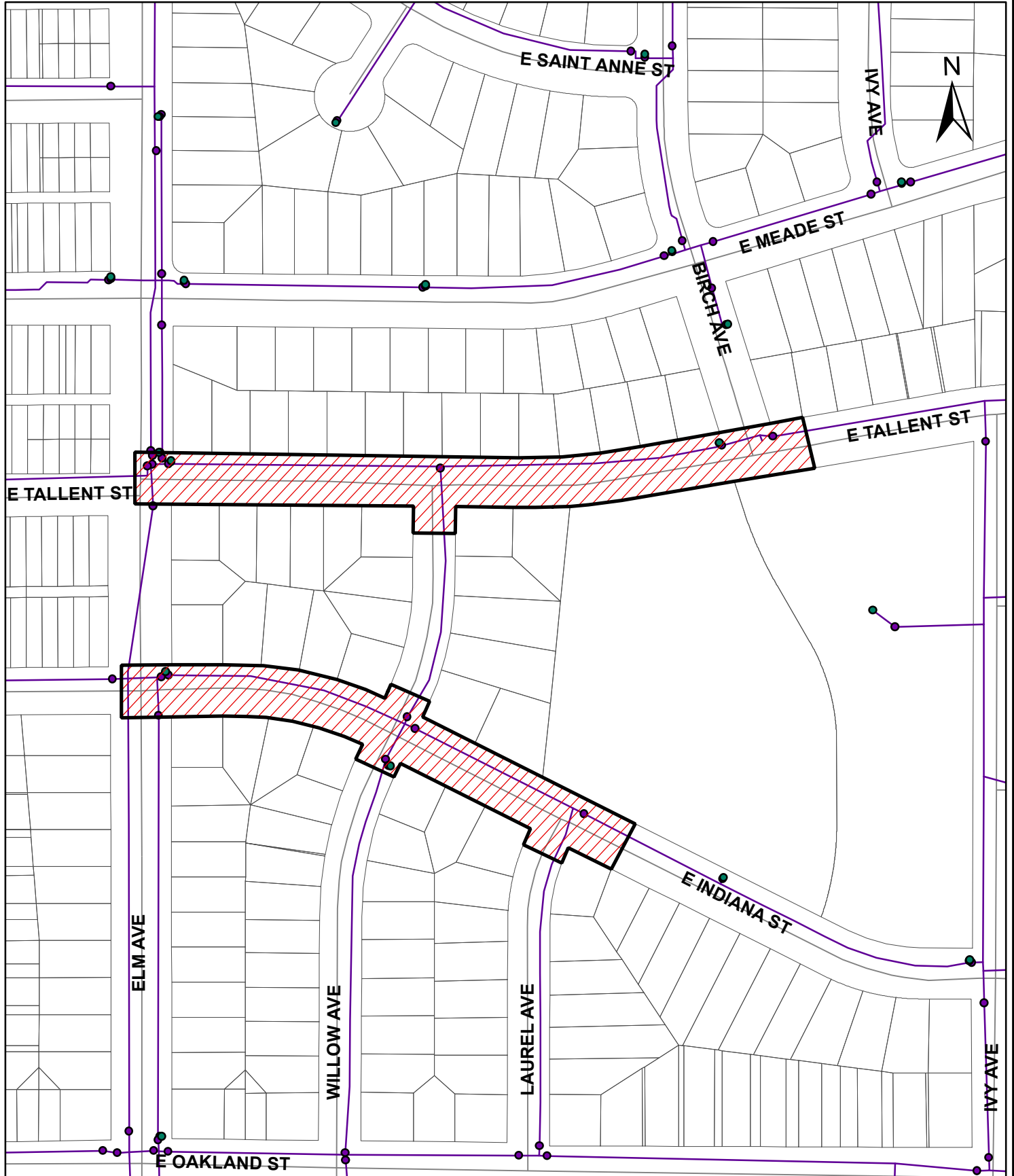
TALLENT STREET & INDIANA STREET WATER MAIN RECONSTRUCTION PROJECT NO. W10-1915 CIP NO. 50845
