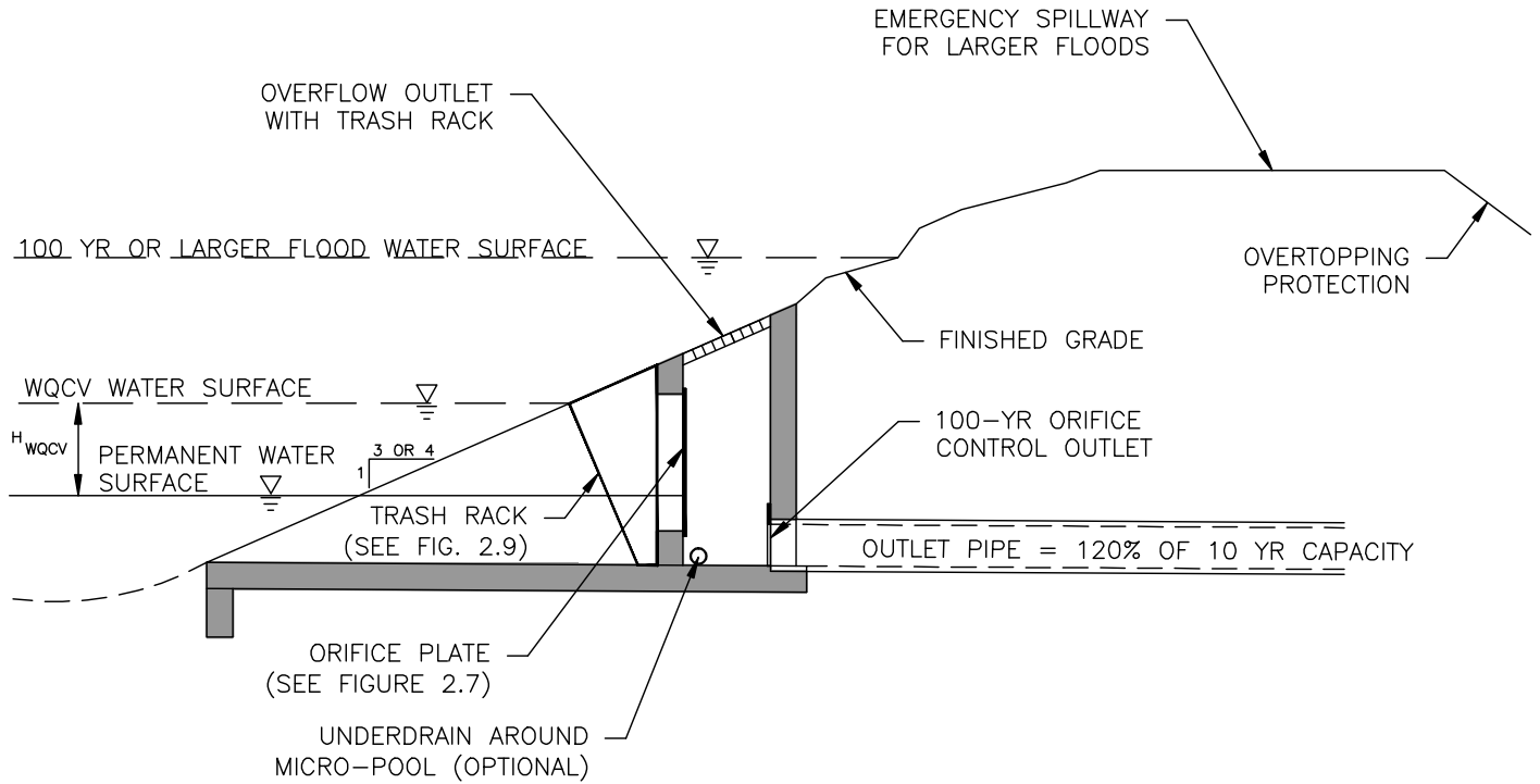
DROP BOX OUTLET OPTION
