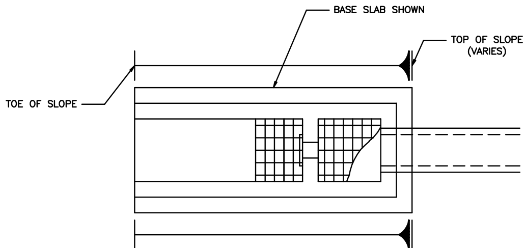
PLAN VIEW—STRAIGHT WINGWALL OPTION
