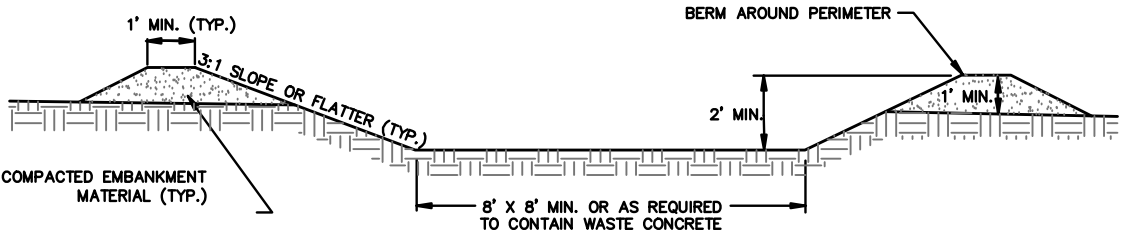
CROSS SECTIONAL VIEW
