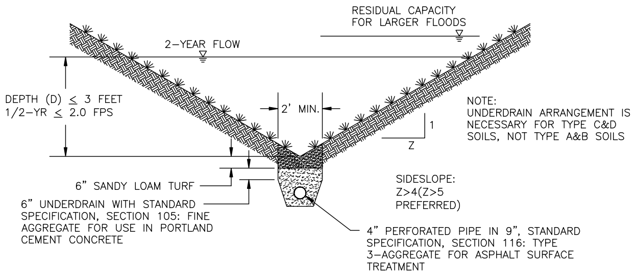
TRIANGULAR GRASS-LINED SWALE SECTION NOT TO SCALE
