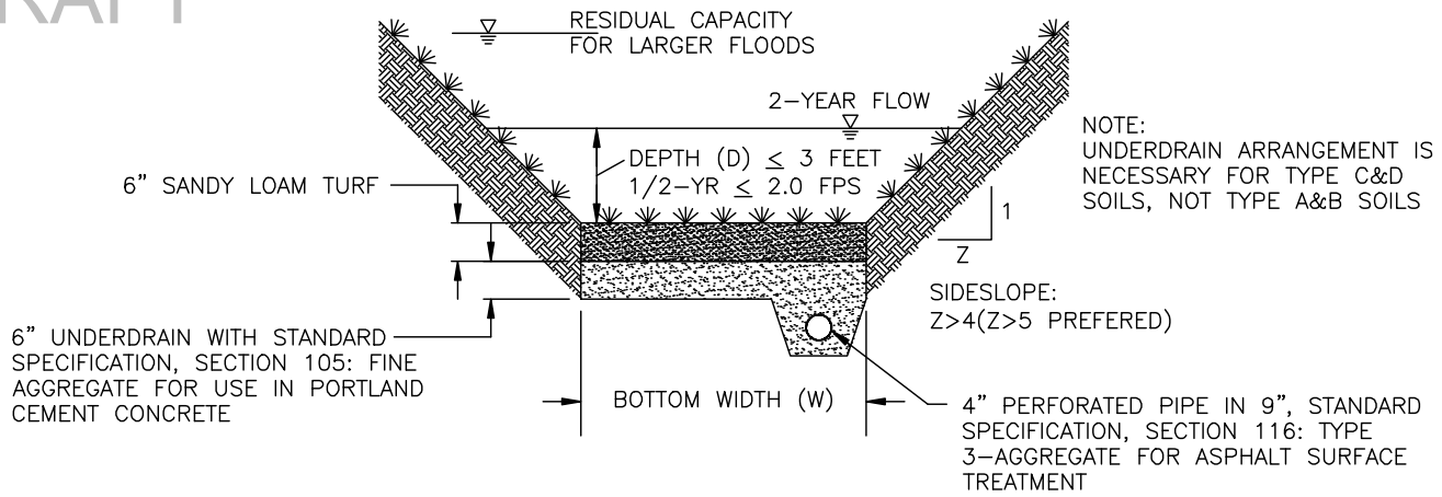
TRAPEZOIDAL GRASS-LINED SWALE SECTION NOT TO SCALE
