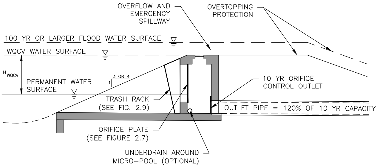
OVERTOPPING SPILLWAY OPTION
