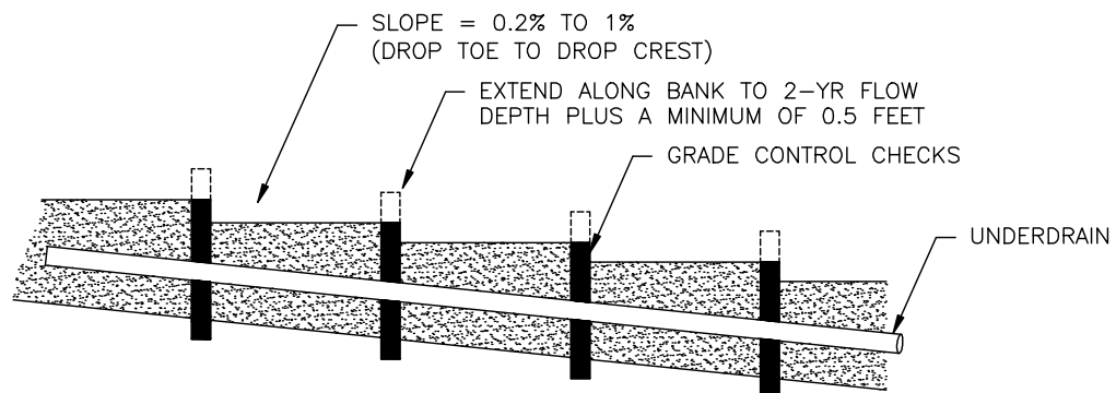
GRASS-LINED SWALE PROFILE NOT TO SCALE
