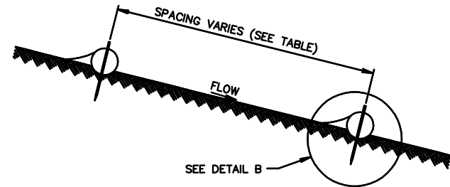
ELEVATION VIEW CUT OR FILL SLOPE INSTALLATION
