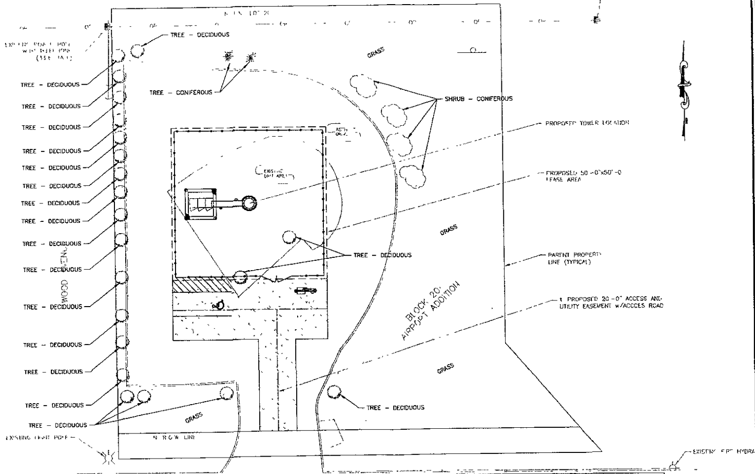
1 LANDSCAPE PLAN SCALE 1"=10'-0"
